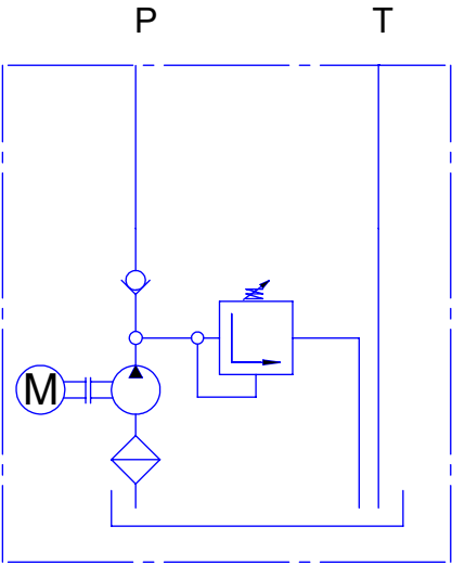
Hydraulic Circuit P, T = G 3/8"
