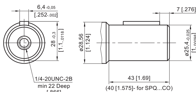
CO - \varnothing 1" straight, Parallel key \frac{1}{4} \times \frac{1}{4} \times 1" BS46 Max. Torque 34 daNm [3010 lb-in]
